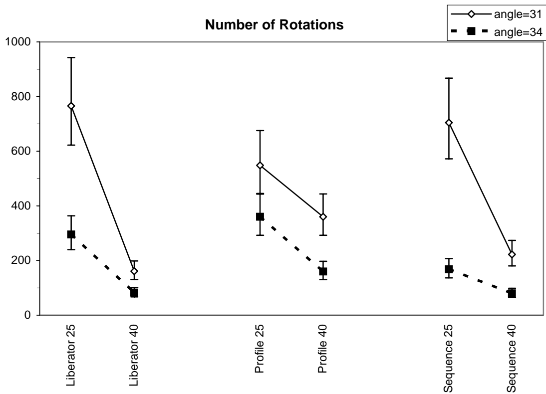
Figure 1 Average Rotations to Failure in the Twelve Experimental Groups
